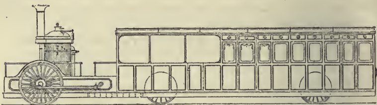
FIG. 49.—THE "FAIRFIELD," ADAMS'S COMBINED BROAD-GAUGE ENGINE AND TRAIN, FOR THE BRISTOL AND EXETER RAILWAY
