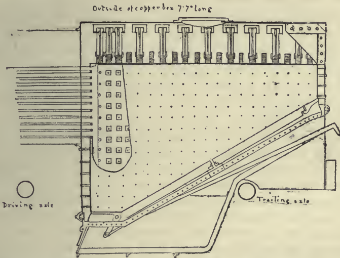
FIG. 77.—CUDWORTH'S SLOPING FIRE GRATE, FOR BURNING COAL, AS FITTED TO SOUTH EASTERN RAILWAY LOCOMOTIVES
