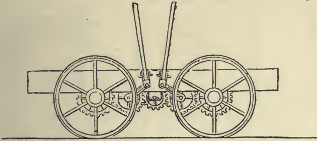
FIG. 6.—STEPHENSON'S INITIAL DRIVING GEAR FOR LOCOMOTIVES
